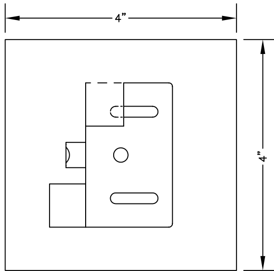
PLAN OF CAP SEAM CLIP W/BEARING PLATE
