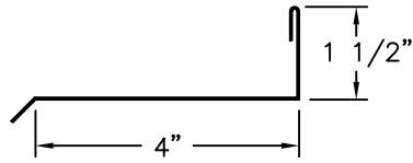
DOOR/WINDOW TRIM
