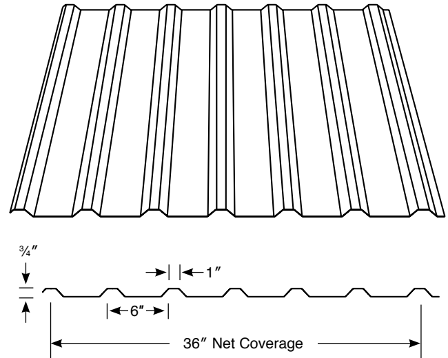
36" Width U-Panel Section Properties
